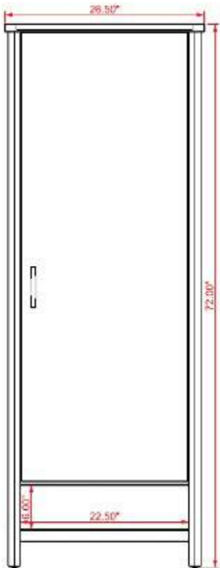
Front Elevation with Right Hand Hinge
