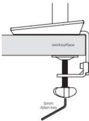
Desk Clamp Detail
