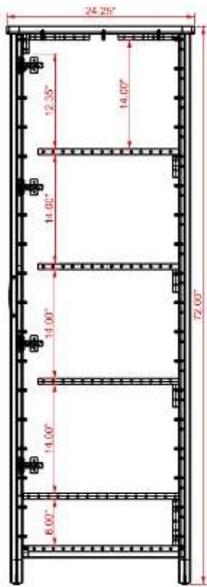
Section Cut - Shelving
